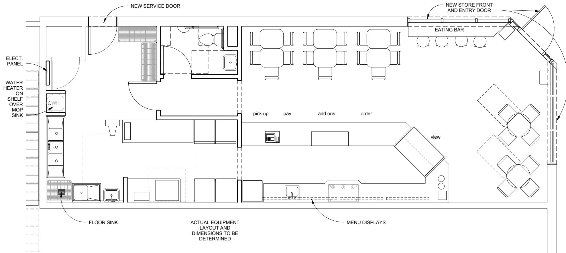
① PRELIMINARY FLOOR PLAN 1/4" = 1'-0"
