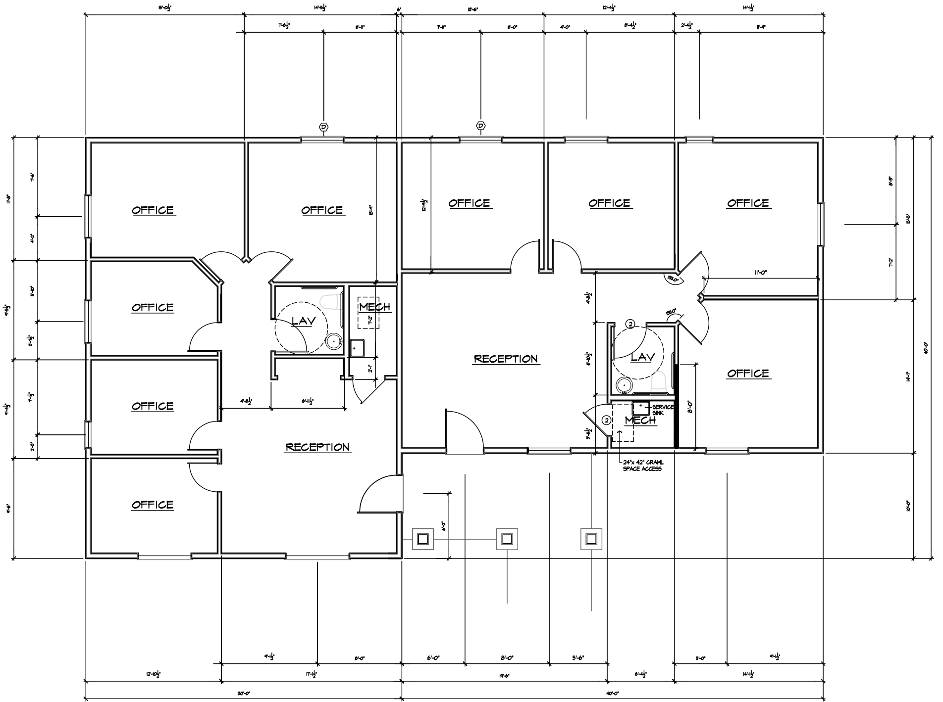
MAIN FLOOR PLAN
